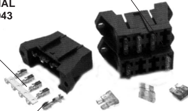
PART# GM-12004943 4 GANG FUSE BLOCK
