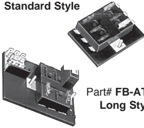
Part# FB-ATC6 Standard Style
