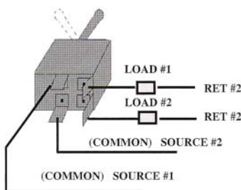
Two Positions On-Off Two single wire circuits
