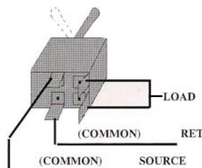
Two Positions On-Off One double wire circuit
